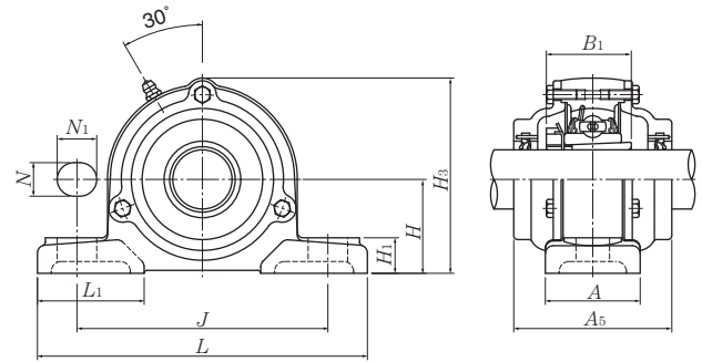
Cast dust cover type (Open end) C-UKP...D1
