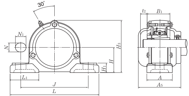
Cast dust cover type (Close end) CM-UKP...D1
