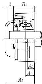
Cast dust cover type (Close end) CM-UKFL...D1
