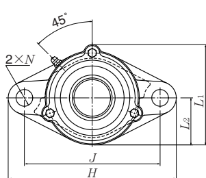
Cast dust cover type (Open end) C-UCFL...D1
