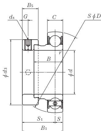
Eccentric locking collar + bearing AEL2xxW3
